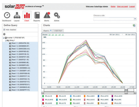
The chart shows the energy output in the form of a graph for every single module in the Exeter installation. The graphs clearly demonstrate the mismatch which exists between modules with different power ratings. Each module still works at its individual MPP since the SolarEdge power optimisers perform MPPT for each module separately.
