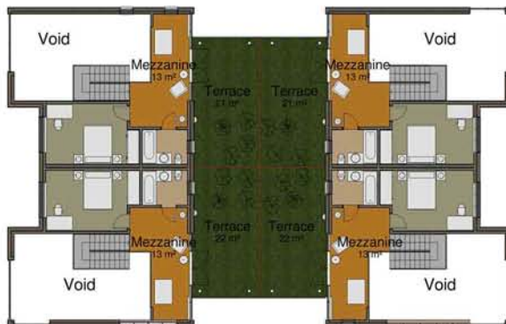
2 Second Floor 1 : 200
