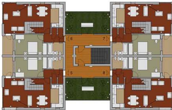
1 First Floor 1 : 200
